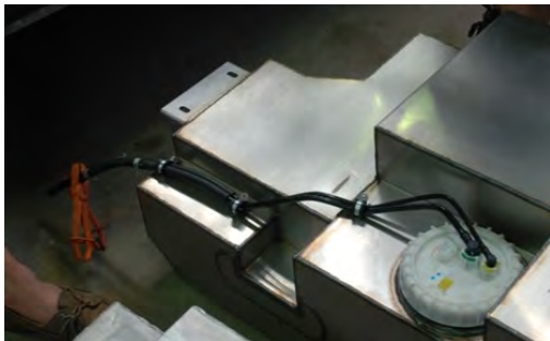
Cushions clamps– used to hold OE fuel lines in place to prevent kinking
